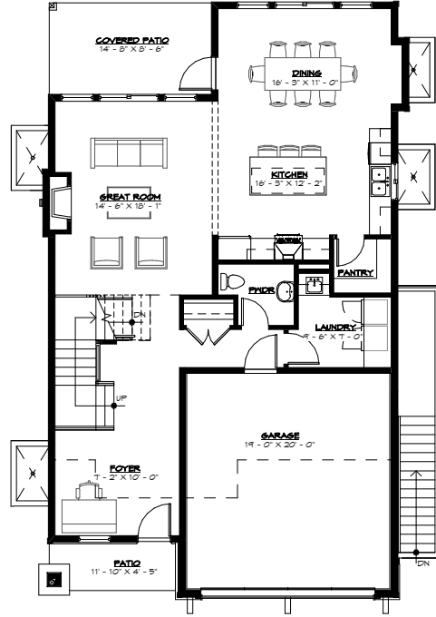
MAIN FLOOR PLAN - C1
