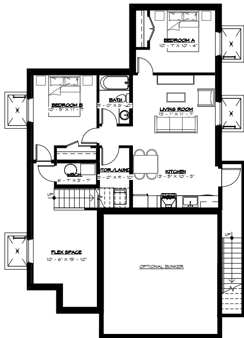
BASEMENT PLAN - B1
