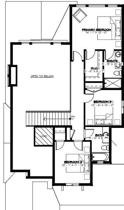
UPPER FLOOR PLAN - B1
